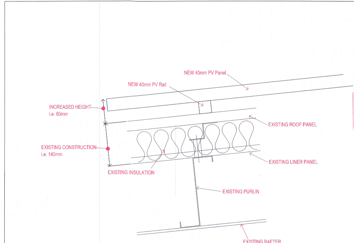
TYPICAL SOUTH ROOF CONSTRUCTION
