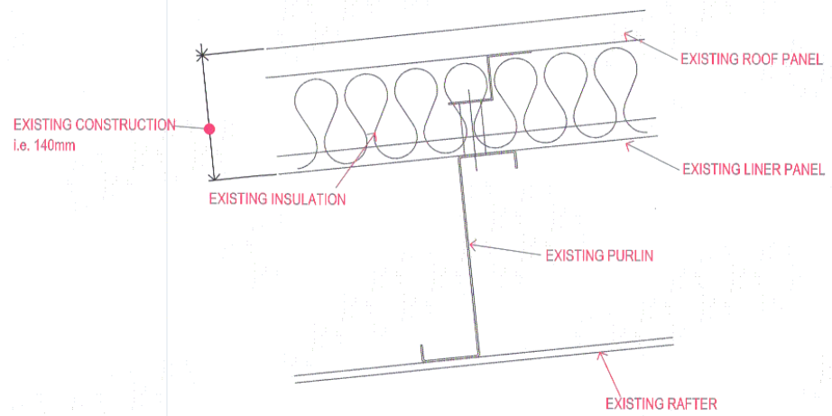
TYPICAL NORTH & SOUTH ROOF CONSTRUCTION
